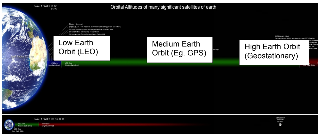
Figure 1 Orbital altitudes
